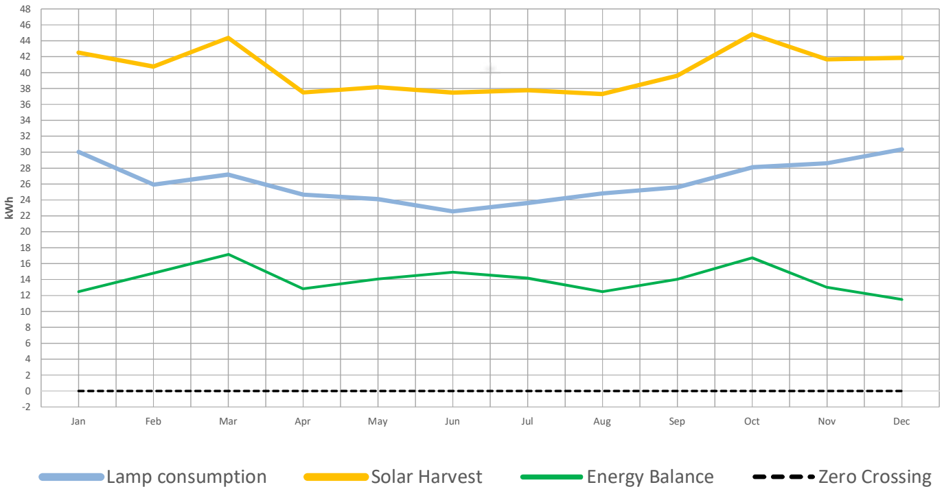
Energy data for Samili 3 with 73W load
